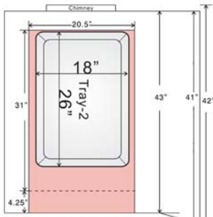
Top View and Baking Chamber Dimensions
